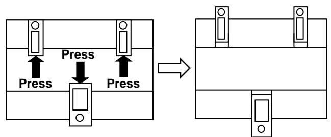
Clips in their original position (for DIN rail mount) Clips in position for wall mount (for DIN rail mount)
